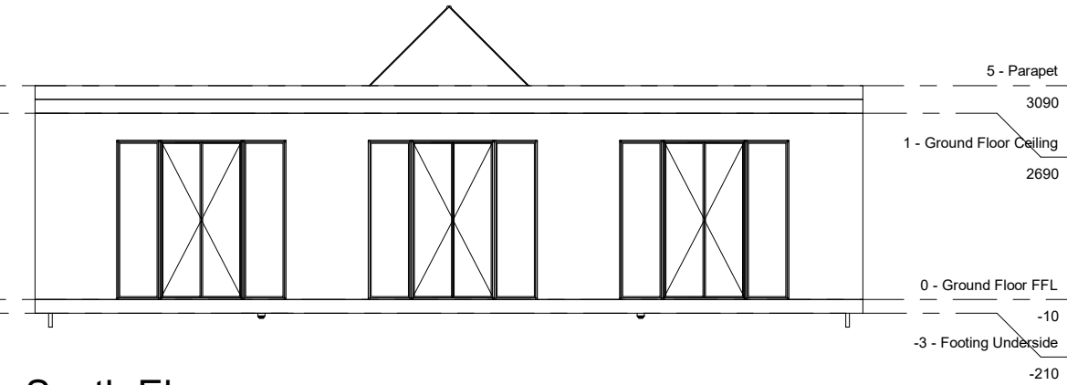
South Elev
