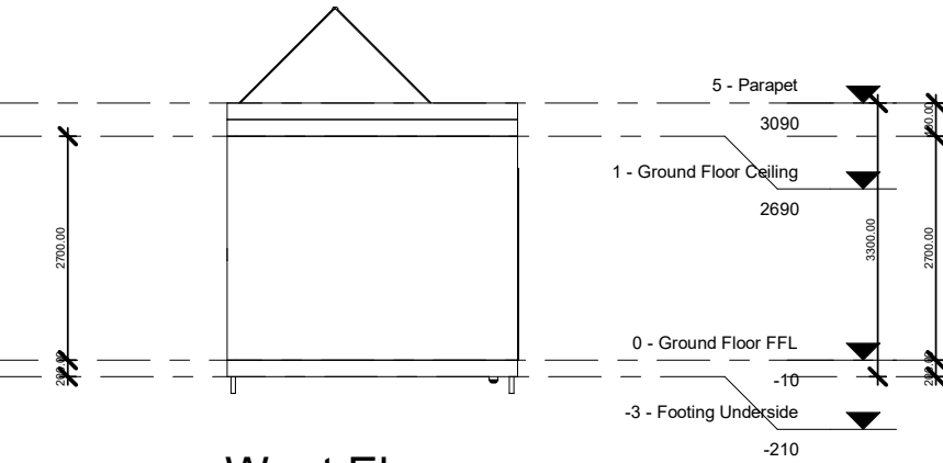
West Elev
