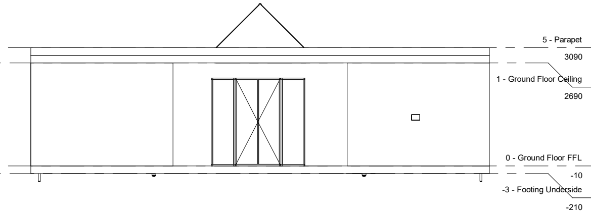
North Elev
