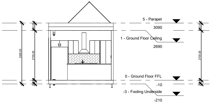
East Elev
