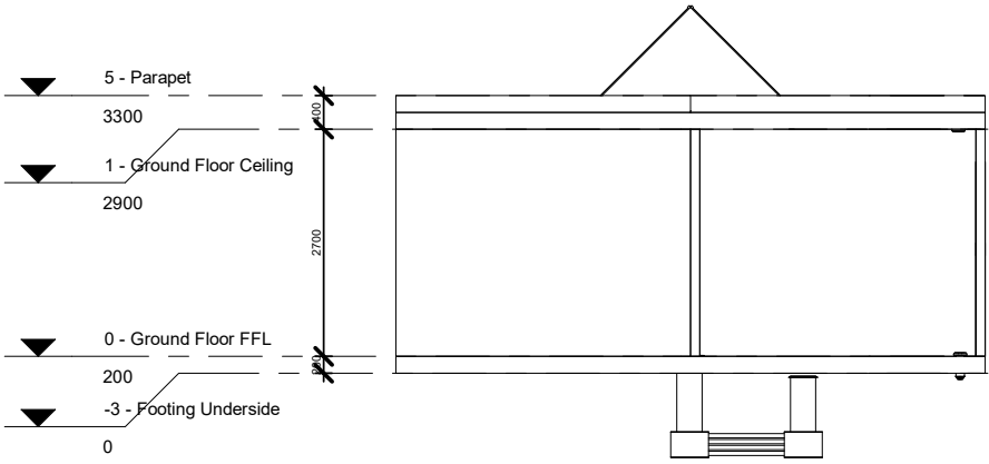
East Elev.
