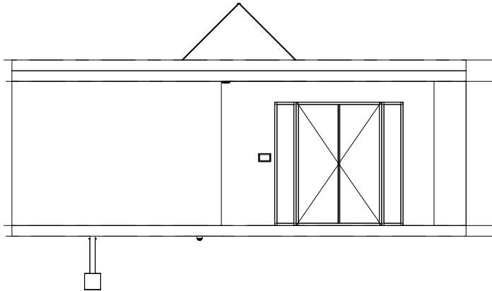
South Elev.
