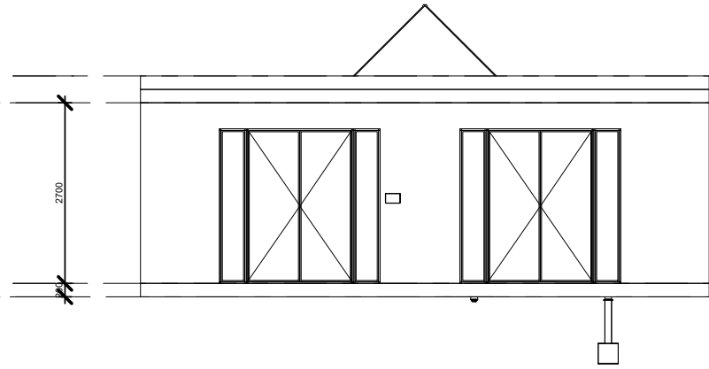
North Elev.
